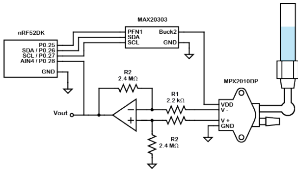
Fig. 5: Basic Hardware Schematic for Example Sensor Application. Only shows used pins on the nRF52 and MAX20303.
