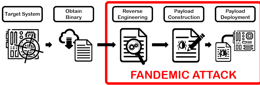
Fig. 3: Overview of the FANDEMIC attack flow. Before beginning the attack, the target device is chosen and original firmware is obtained. The FANDEMIC attack starts with reverse engineering the binary to determine PMIC configuration information. The next stage is firmware modification, and the final stage is firmware deployment.
