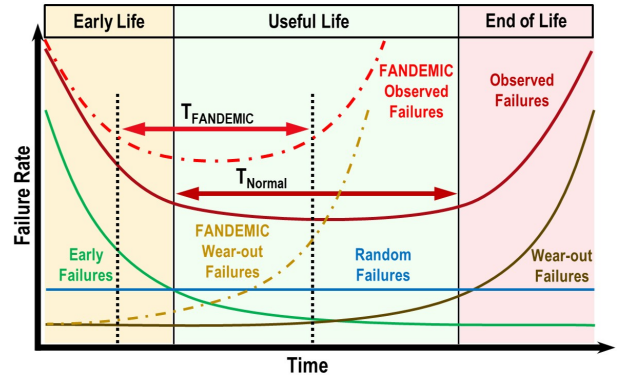
Fig. 8: Expected behavior of the life cycle of logic circuits in presence of FANDEMIC vs. Normal conditions. The red solid line shows the expected life cycle of IC components, and the red dashed line depicts the estimated behavior caused due to FANDEMIC ( T_{FANDEMIC} < T_{Normal} ). The brown solid line shows the normal wear-out failures, and the gold dashed line shows the wear-out failures caused by FANDEMIC. Additionally, the solid blue line and solid green lines represent the random failures and early failures, respectively.
