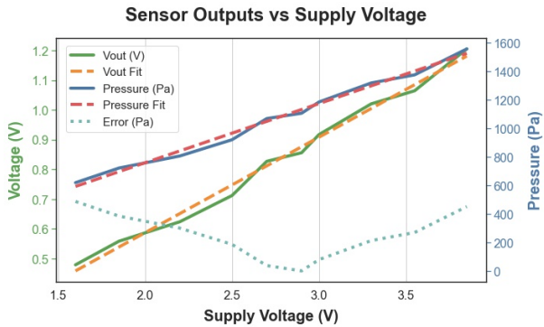
Fig. 7: Sensor output voltage, pressure reading, and pressure error relative to the original voltage of 2.9V (arbitrary), all as a function of the supply voltage. The slope of the dashed red fit regression line is 414.73 Pa/V and the slope of the dashed orange regression line is 0.321 V/V.
